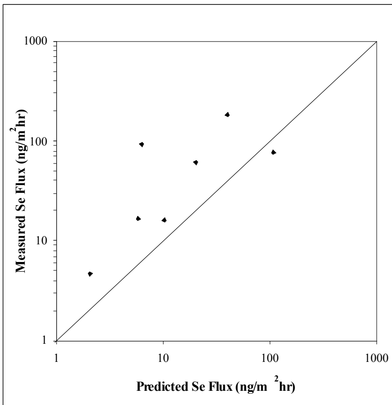
Figure 16d. Relationship between Estuarine model predicted volatilization rates to measured volatilization rates after corrections for background and measurement inefficiency. Top: log axes. Bottom: linear axes
