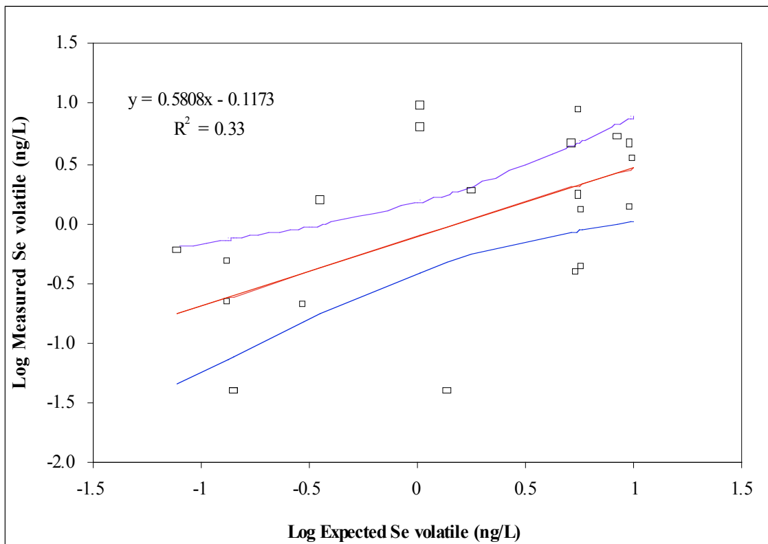
Figure 17d. Determination of the 95% confidence interval using expected vs. measured data of near surface volatile Se concentrations. Expected values obtained from the sinusoidal function. Top: log values in a normal scale. Bottom: Arithmetic values in a log scale.
