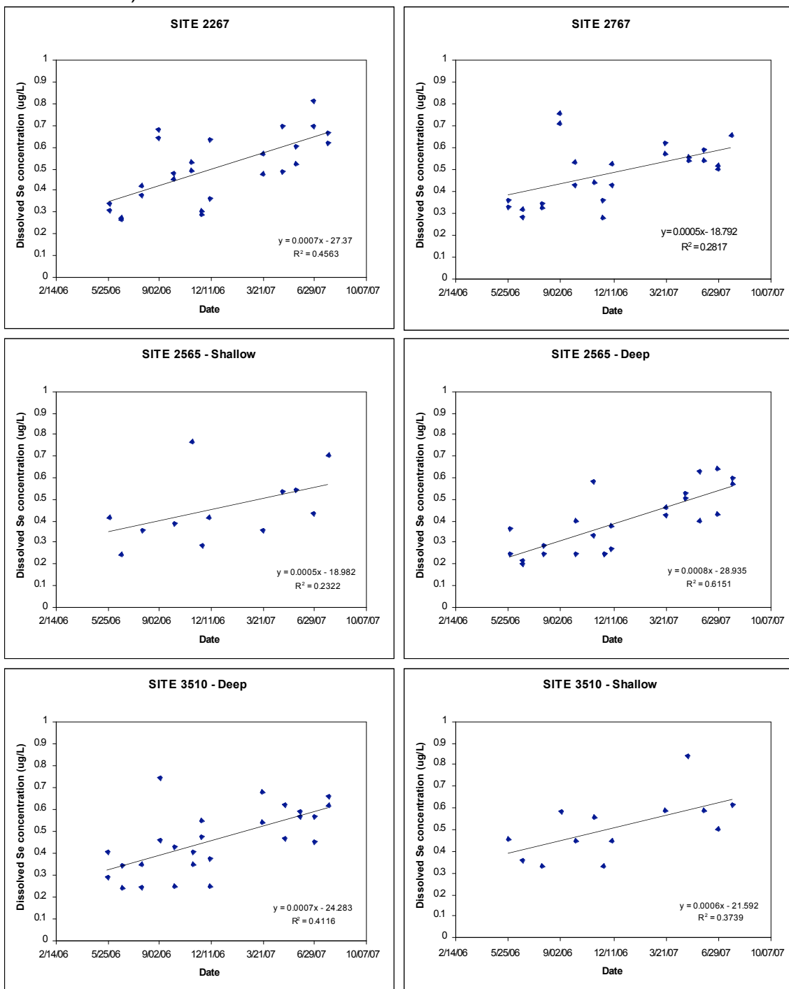
Figure 41a. Dissolved Se concentration trajectories (data from Frontier Geosciences).
