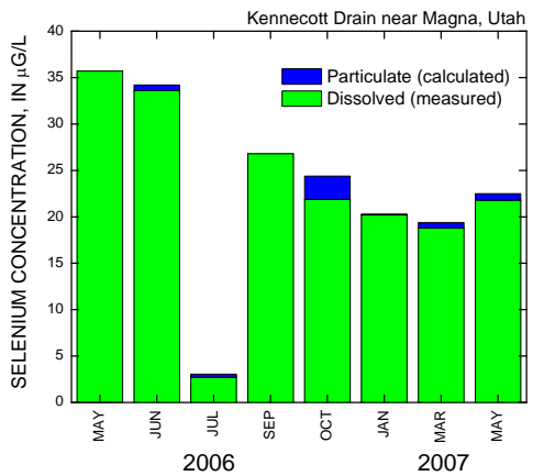
Figure 22. Distribution of dissolved and particulate selenium in water samples collected from inflow sites to Great Salt Lake during May 2006 through July 2007. Note the difference in scale for the KUCC Drain in comparison to other sites.
