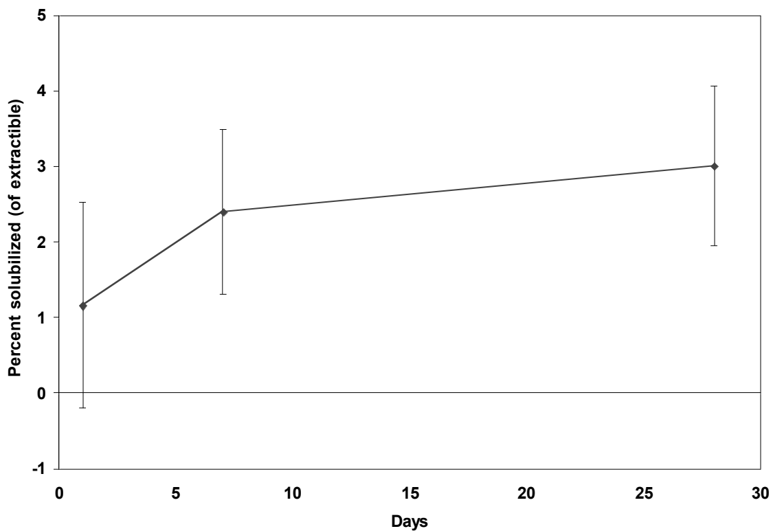
Figure 37b. Time series variation of average percent Se solubilized (of extractable) from all batch equilibration experiments. Bars represent one standard deviation on both sides of the average value.
