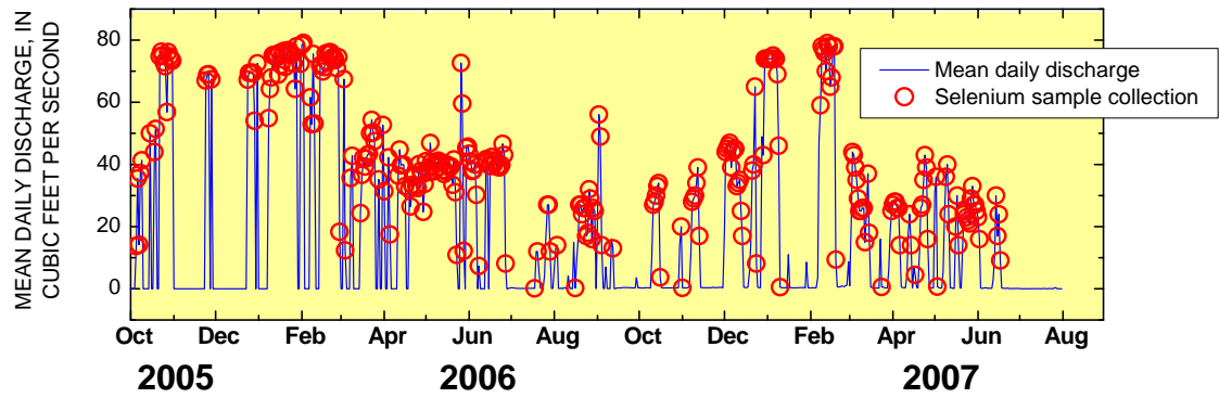
Figure 8. Stream discharge and dates when selenium samples were collected at the KUCC gaging station. Discharge and selenium data prior to June 30, 2006 provided by KUCC (K. Payne, written commun., 2006). Selenium data after June 30, 2006 provided by KUCC and USGS.
