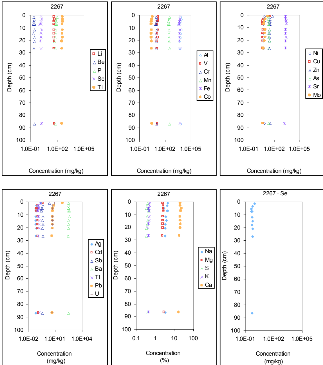
Figure 30. Major and minor elements distribution at site 2267 core
