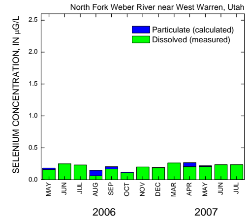
Figure 22. Distribution of dissolved and particulate selenium in water samples collected from inflow sites to Great Salt Lake during May 2006 through July 2007. Note the difference in scale for the KUCC Drain in comparison to other sites.
