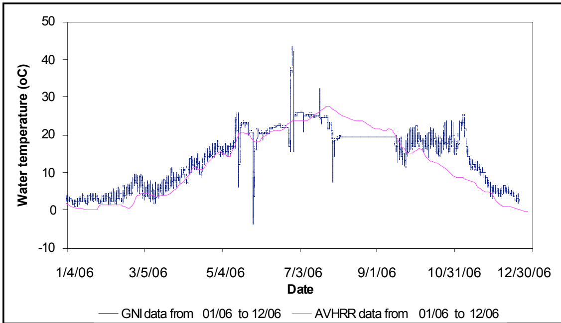
Figure 3c. AVHRR temperature compared with measured temperature at Gunnison Island weather station from January to December 2006 (top). Same comparison for Gunnison Island temperatures from September 2006 to August 2007 (bottom) with the AVHRR data from 2006.
