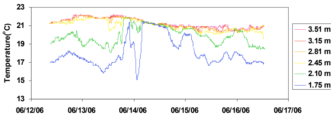
Figure 32a. June temperature record from site 2565, tick marks represent midnight (MDT) and values represent distance above lake bottom. Lowest figure shows wind speed (black) and wind direction (orange) at Hat Island.
