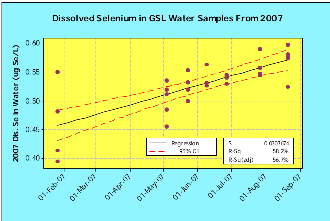
Figure 61. Dissolved selenium in filtered GSL water samples collected from January 2007 to August 2007. A regression analysis of within year selenium concentration in water samples provides an improved interpretation and analysis of the trends.
