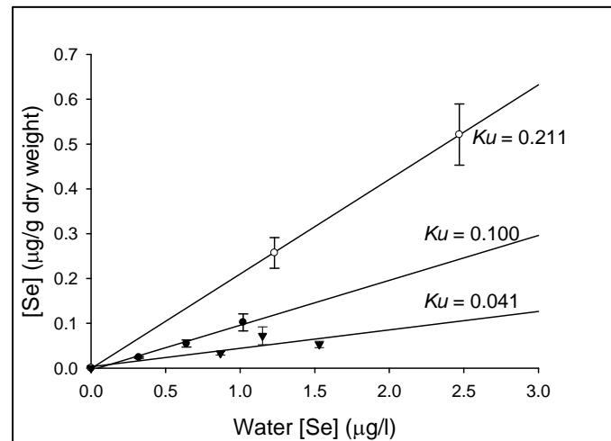
Fig. 8. Selenium uptake by Artemia from the water. Comparison of a subset of data presented in Fig. 7. focusing on low ambient selenium concentrations (open symbols) to the second replicate experiments in artificial GSL medium employing more environmentally realistic selenium concentration (filled circles). Selenium accumulation in Artemia exposed to similar selenium concentrations in natural GSL water (filled triangles) is lower than corresponding uptake in artificial medium.
