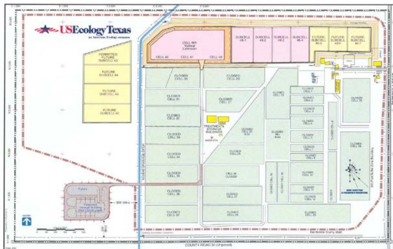
Figure B-16. Robstown, TX Disposal Cell Configuration
