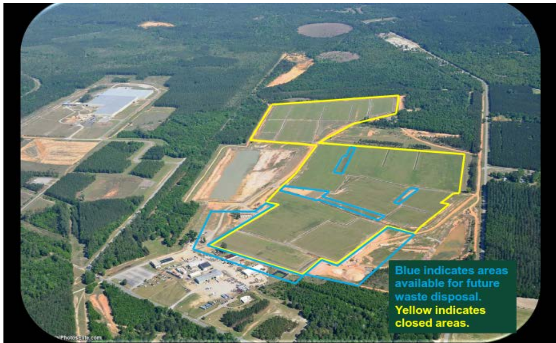
Figure C-29. Aerial Photograph of Barnwell, SC Facility (Source: EnergySolutions 2013)
