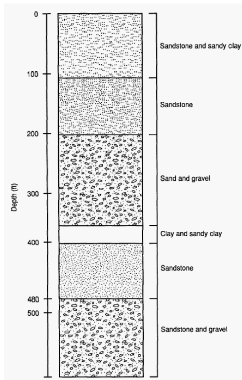
Figure C-28. Barnwell, SC Geology
