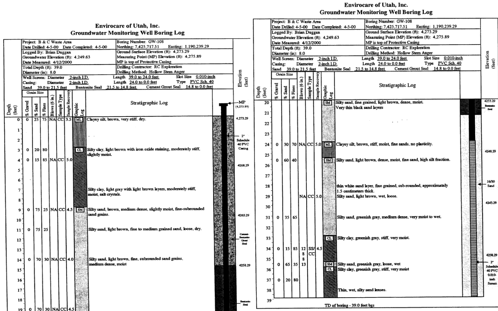
Figure C-18. Clive, UT Geology - Well GW-108
