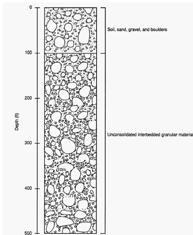
Figure C-23. Hanford, WA Geology
