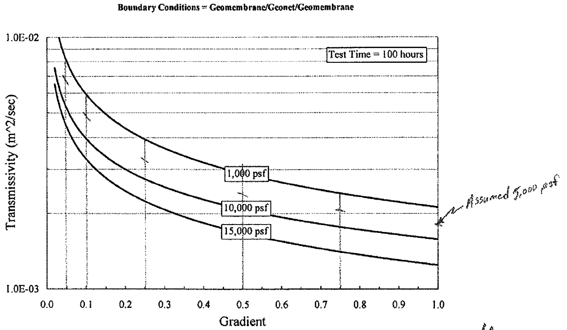
Figure A-7 100-hour transmissivity data for a 300 mil biplanar geonet between two geomembranes.
