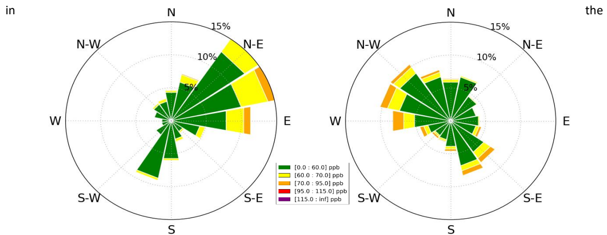
Figure 6. Pollution roses (fraction of time ozone concentrations are in range bins as a function of wind direction) at Badger Island (left) and Farmington Bay (right).
