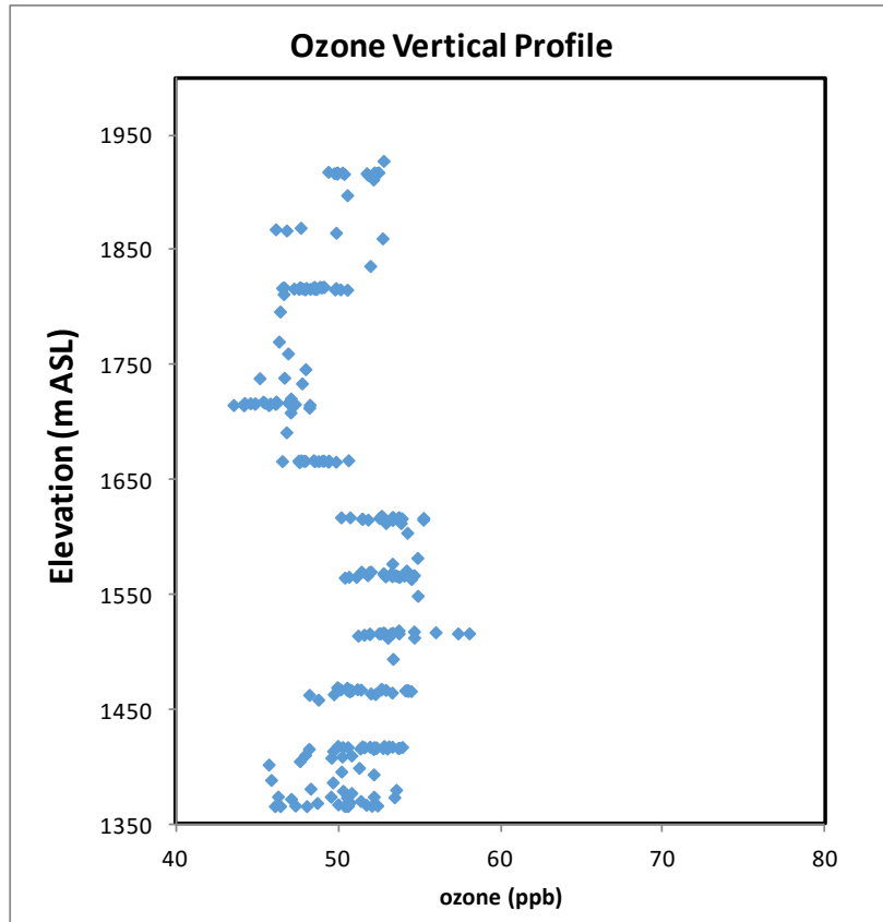
Figure 2. USU's UAV-derived vertical ozone profile, Promontory Point, 16 July 2015, 1202-1245 MDT.
