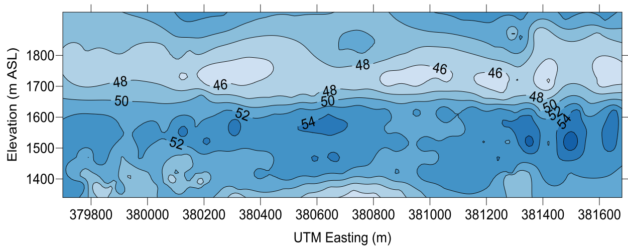
Figure 3. Contour plot of USU's UAV-derived vertical and horizontal ozone transects, Promontory Point, 16 July 2015, 1202-1245 MDT.
