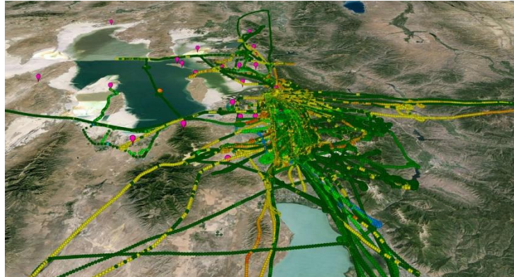
Figure 9. Summary of the spatial distribution of all the observations collected during GLSO 3 S. The ozone sensor deployed on the KSL traffic helicopter provided many of the tracks extending away from the Wasatch Front.
