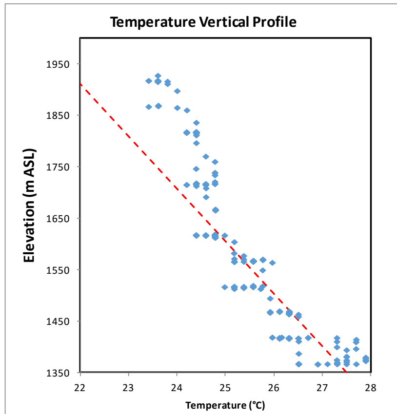
Figure 1. USU’s UAV-derived vertical temperature profile, Promontory Point, 16 July 2015, 1202-1245 MDT.
