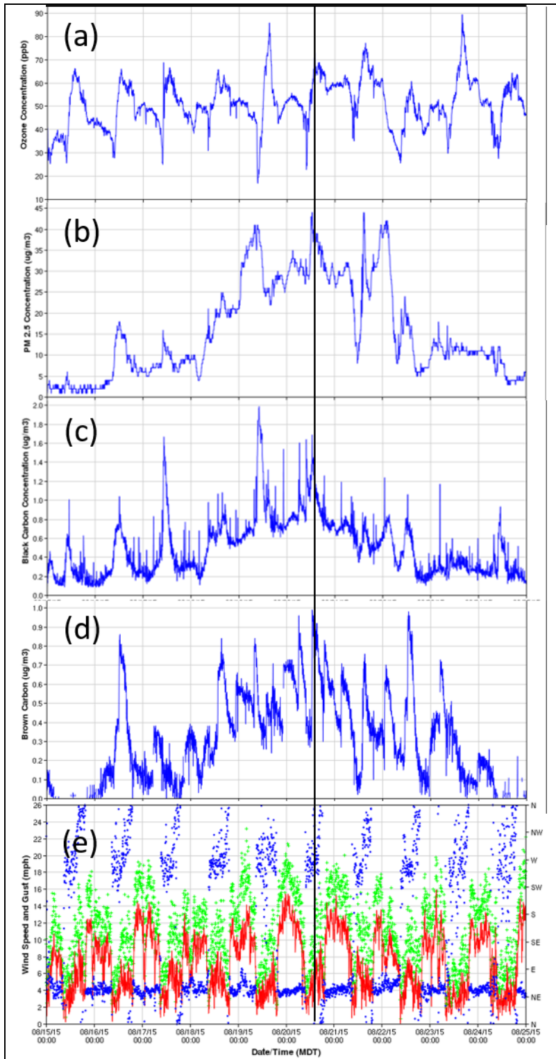
Figure 16. Conditions on the University of Utah campus from 15-24 Aug 2015 of: a) ozone; b) PM 2.5 ; c) black carbon; d) brown carbon UV-BC; e) wind speed (red), gust (green); direction (blue). The black vertical line denotes 1730 MDT 20 August for reference.
