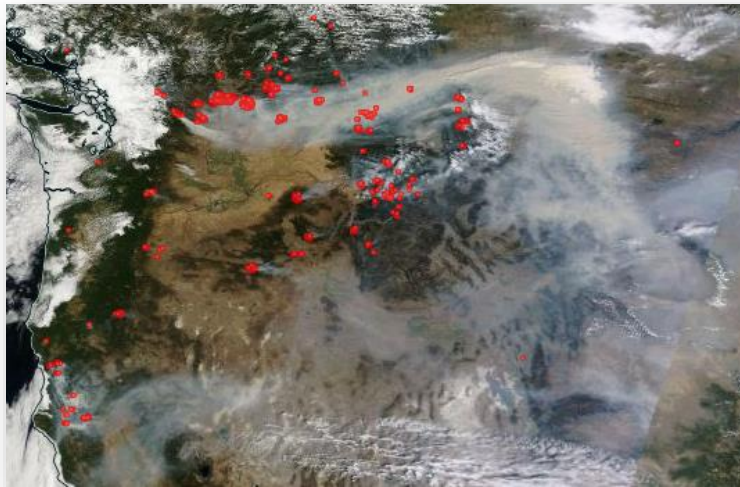
Figure 13. MODIS image of smoke transport on 20 August 2015.
