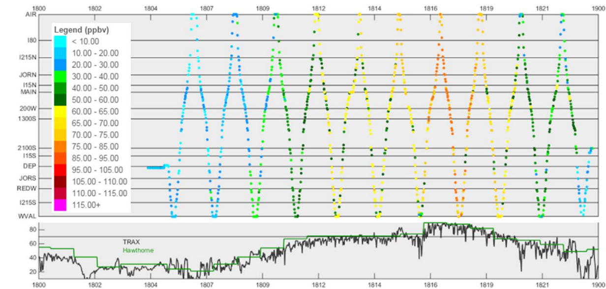
Figure 10. Top. Ozone concentration from sensor on TRAX light rail car travelling on 18 June on the Green Line from the Airport (AIR) to West Valley (WVAL) as a function of time in MDT along the horizontal axis. Bottom. Comparison of ozone on the light rail car (black) and at Hawthorne (green).
