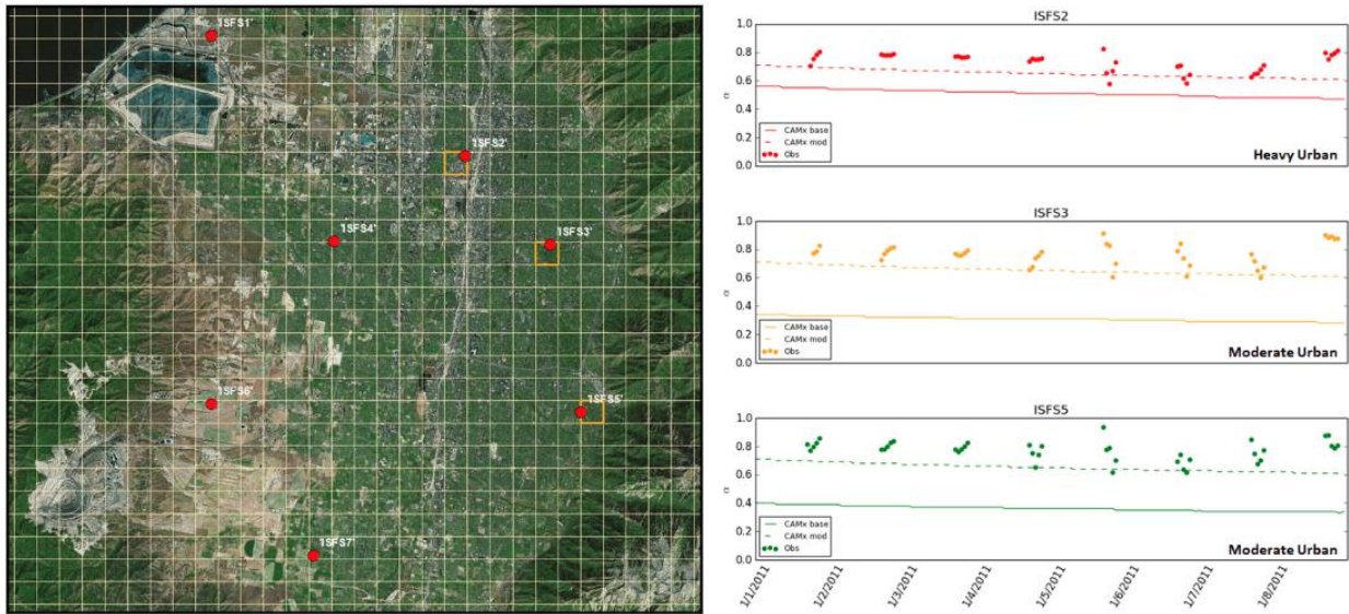
Figure 3. Left) Map of University of Utah surface radiation monitoring stations during January 2011 field monitoring study. Red dots show 7 monitor locations. Orange squares highlight model domain 1.33 km grid-cells collocated with 3 urban monitors. Right) For each of 3 urban monitors, dots show albedo measurements derived from observed radiation flux for January 1-8, 2011. Solid lines show default CAMx albedo at grid-cells collocated with each of the 3 urban monitors. Dashed lines show CAMx albedo after model modification.
