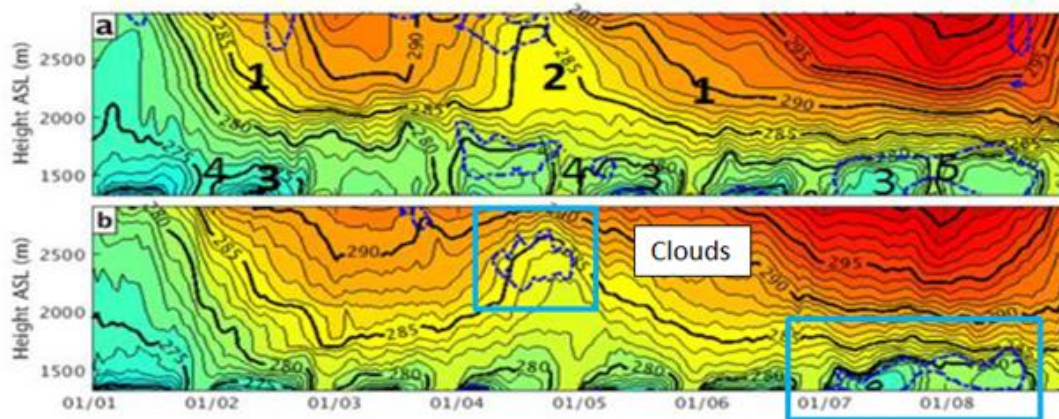
Figure 5. a) Observed potential temperature (K) and RH (90% threshold, dashed blue line) b) Modeled potential temperature (K) and cloud water mixing ratio (0.1 g kg -1 threshold, dashed blue line) in Salt Lake Valley. Courtesy of Erik Crosman, University of Utah.
