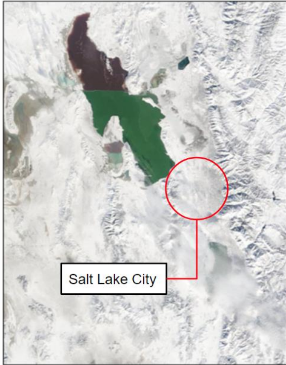
Figure 2. January 1, 2011 MODIS satellite imagery from the Terra platform centered over the GSL and SLV. Red Circle indicates Salt Lake City metropolitan area.
