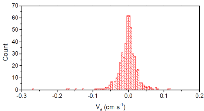
Figure 6. Histogram of ozone deposition velocity calculations for the snow-covered period (early February, 2013) inclusive of both nighttime and daytime data. Mean and median ozone deposition velocity were -0.002 and 0 cm s -1 , respectively.
