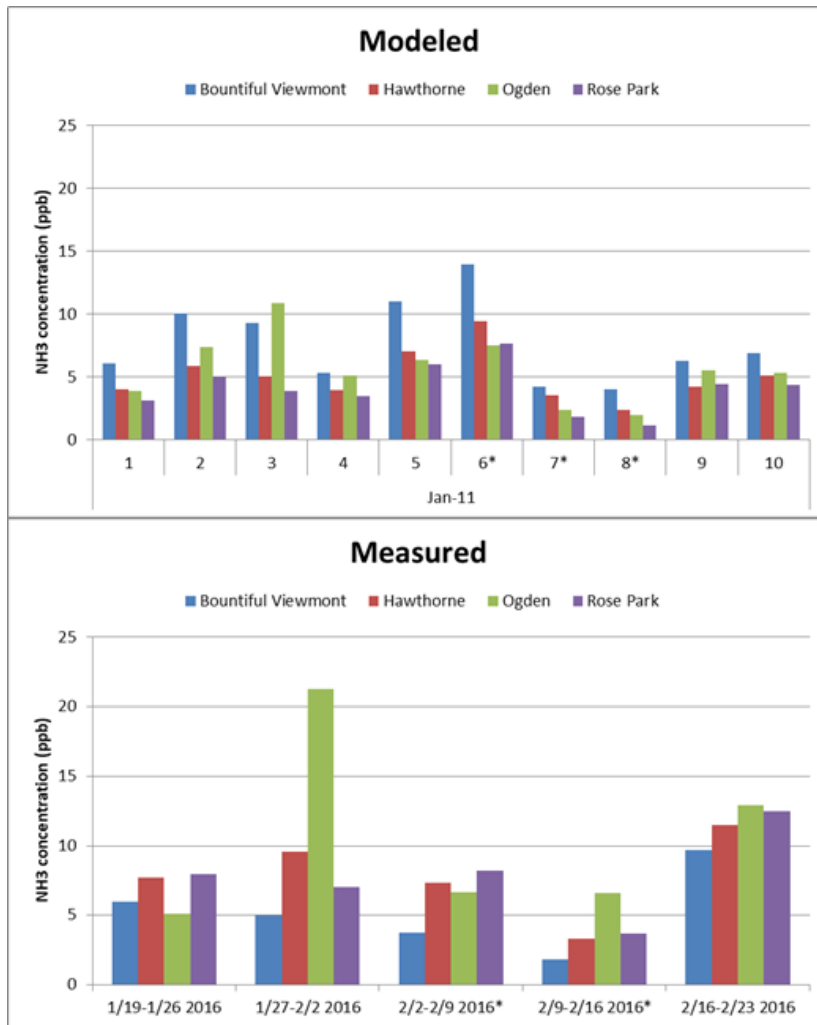
Figure 1. Top panel) Daily-averaged modeled ammonia for January 1-10 2011. Asterisks note days where modeled 24-hour PM_{2.5} was greater than 35 \mu\text{g}/\text{m}^3 . Bottom panel) Seven-day averaged measured ammonia for January 19 - February 23, 2016. Asterisks note weeks where measured PM_{2.5} was greater than 35 \mu\text{g}/\text{m}^3 for most of that week.
