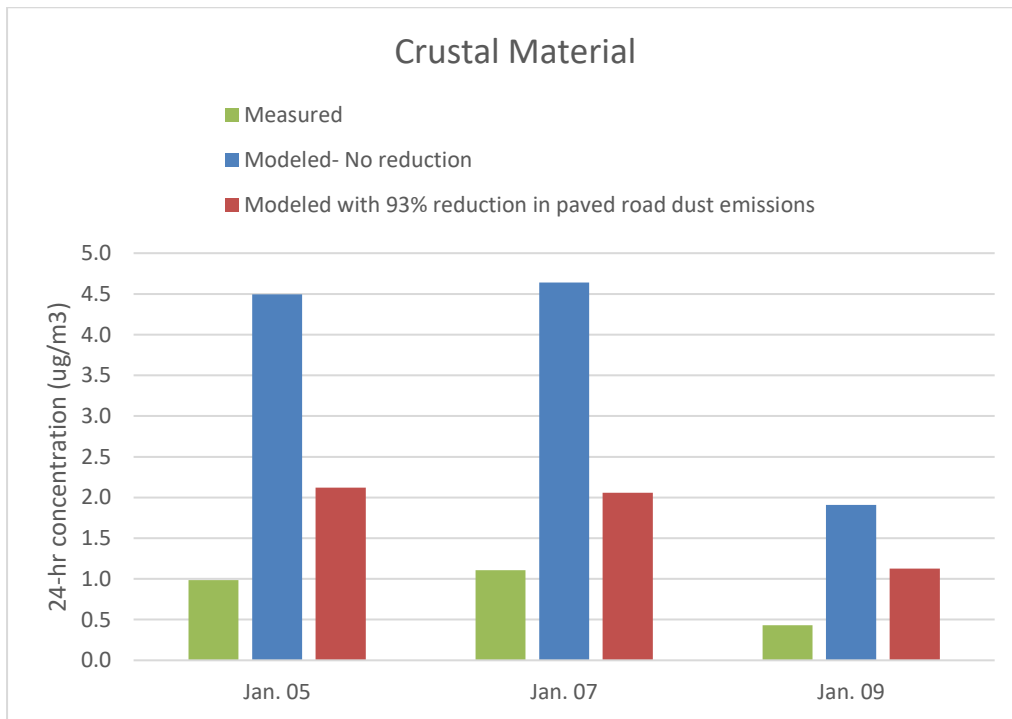
Figure 7. Measured and modeled crustal material concentration following the reduction of paved road dust emissions by 93%.
