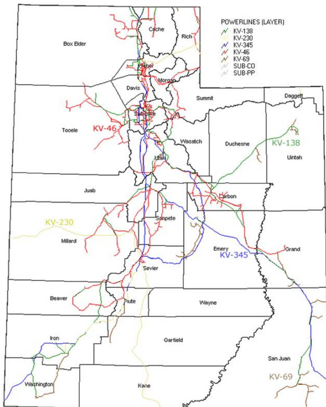
Figure 5 - Utah's Transmission and Distribution Network
