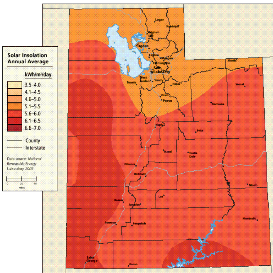
Figure 12 - Solar Energy Potential in Utah
