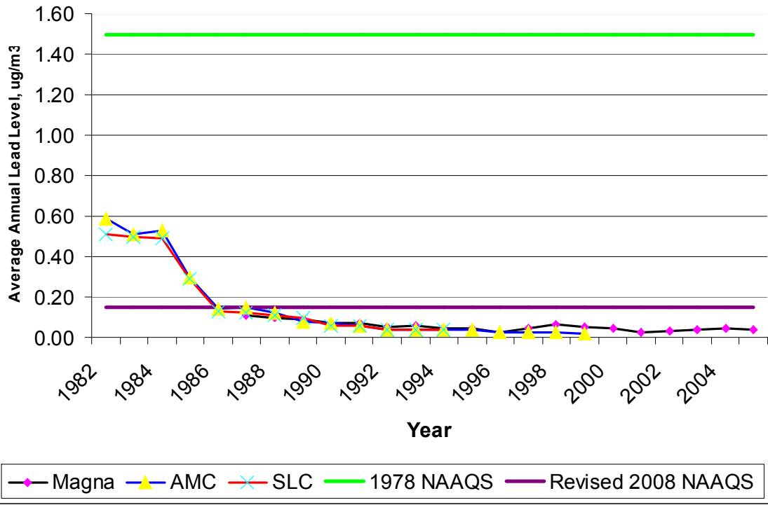
Trends in Ambient Air Lead Concentration: 1982-2005
